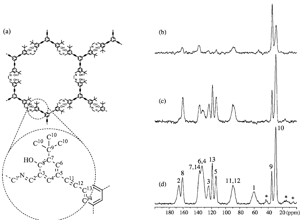
Figure 1. (a) Fragment of an ideal hexagonal structure of salen polymer 2 and assignment of the carbon atoms in the asymmetric unit; (b)–(d) ^{13}\text{C}\{^1\text{H}\} MAS NMR spectra (7.05 T) of 2 recorded with a spinning speed of 9.0 kHz; (b) spin-echo MAS spectrum obtained without decoupling during the echo period ( 2\tau = 7.14 \text{ ms} ), a 15 s repetition delay, and 5200 scans; (c) cross-polarization-depolarization (CPD) MAS spectrum recorded with a CP contact time of 5.0 ms, a CPD depolarization time of 80 \mu\text{s} , a repetition delay of 5 s, and 1024 scans; (d) standard CP/MAS NMR spectrum obtained with a CP contact time of 5.0 ms, a repetition delay of 5 s, and 2048 scans; the asterisks indicate spinning sidebands while the numbers give the assignment of the resonances to the individual carbon atoms in the asymmetric unit shown in part (a)
